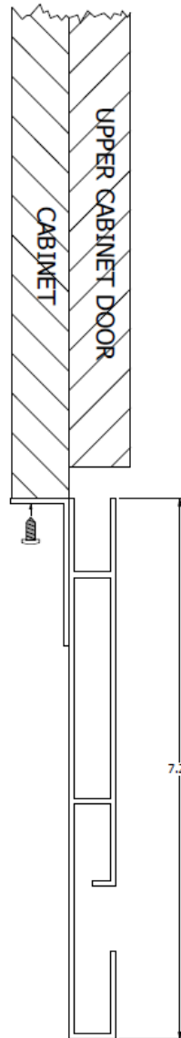
TOP TRIM PIECE (SIDE VIEW)
