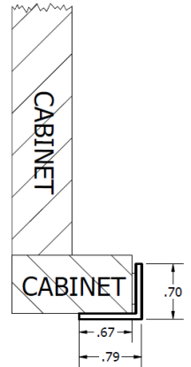
SIDE TRIM PIECE (TOP VIEW)
