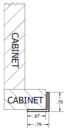
SIDE TRIM PIECE (TOP VIEW)
