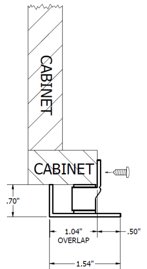
SIDE TRIM PIECE (TOP VIEW)
