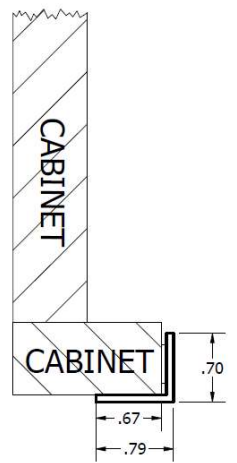
SIDE TRIM PIECE (TOP VIEW)
