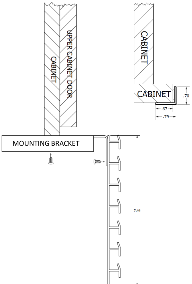
TOP TRIM PIECE (SIDE VIEW)
