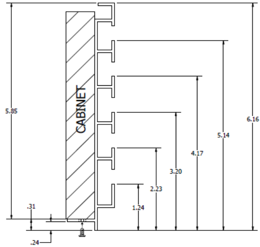
SIDE TRIM PIECE DETAILS (TOP VIEW / NOT TO SCALE)
