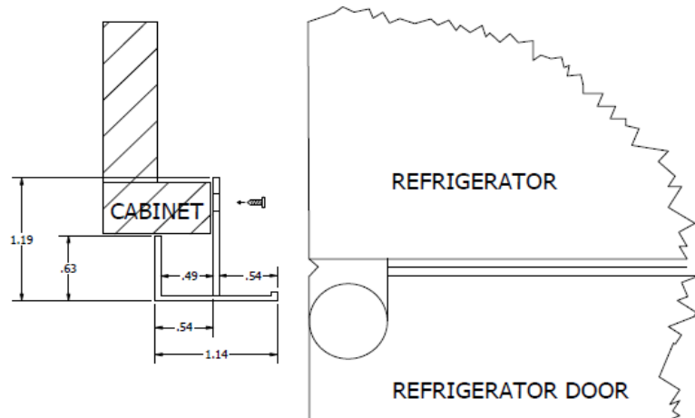
SIDE TRIM PIECE DETAILS (TOP VIEW / NOT TO SCALE)
